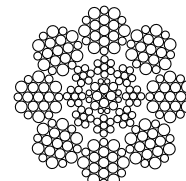
80-094 8 x 19 PAWO 819W Warrington with full steel core (IWRC)
