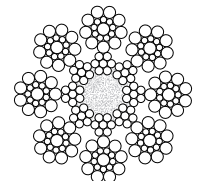
80-045 8 x 19 PAWO F3 Seale with steel-reinforced natural fiber core
