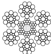
80-086 and 80-043 6 x 19 PAWO F3 Seale with steel-reinforced natural fiber core
